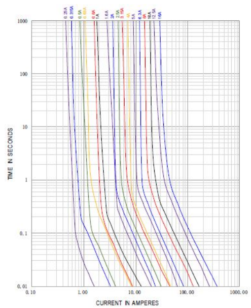
Average Time Current (I-T) Curves
